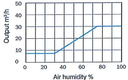
Air flow vs. humidity chart @ 10Pa.
